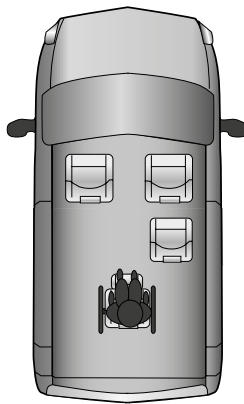
Maximum wheelchair width with 1 rear seat 695mm
