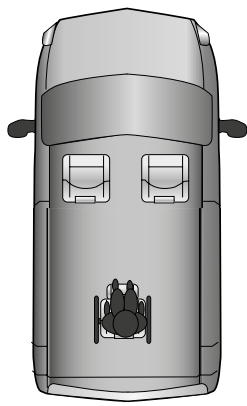
Maximum wheelchair width with 0 rear seats 795mm
